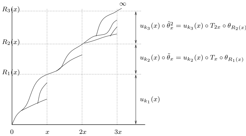
FIG. 1. An example with k_1 = 3, k_2 = 2 and k_3 = 4 .
