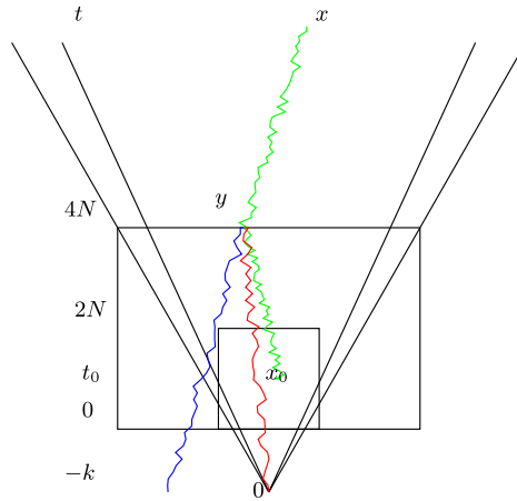
FIG. 2. Coupling from the past.
