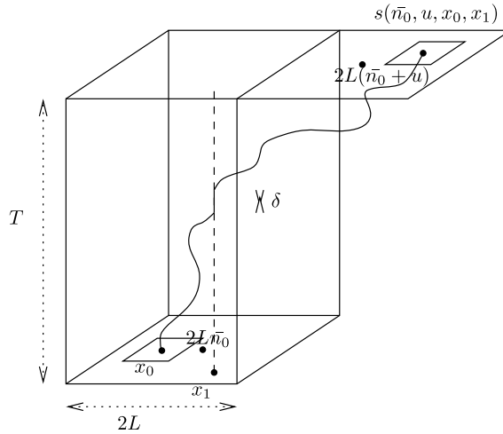
FIG. 1. The good event A(\bar{n}_0, u, x_0, x_1) .
